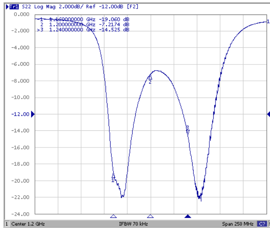
S22
